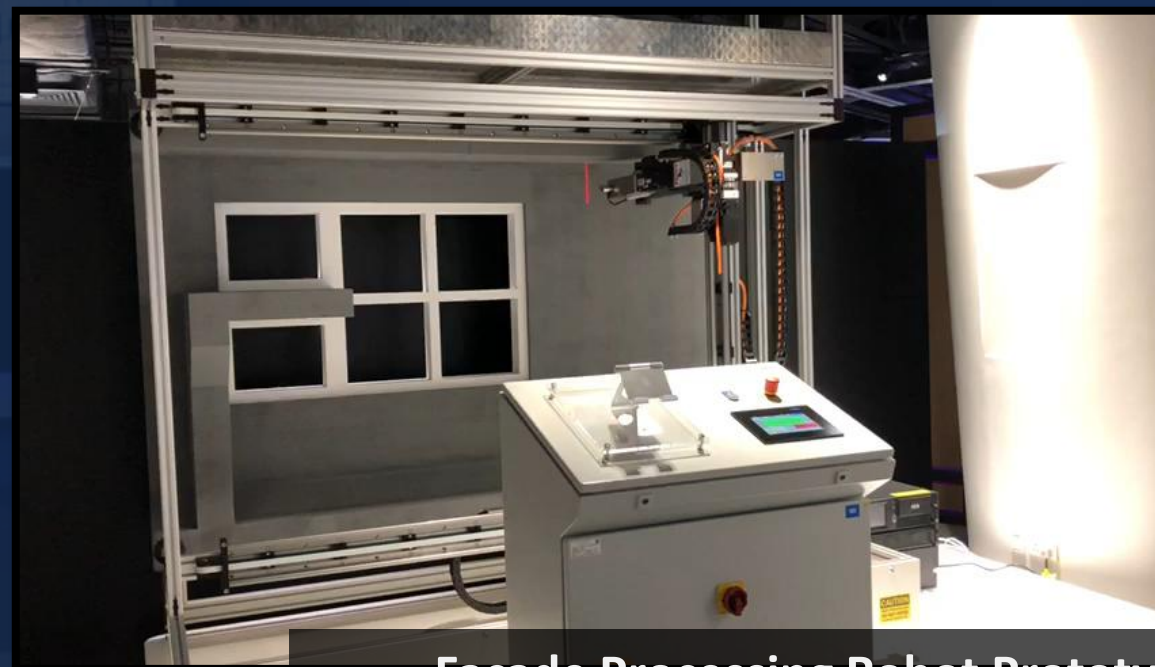
Facade Processing Robot Prototype
